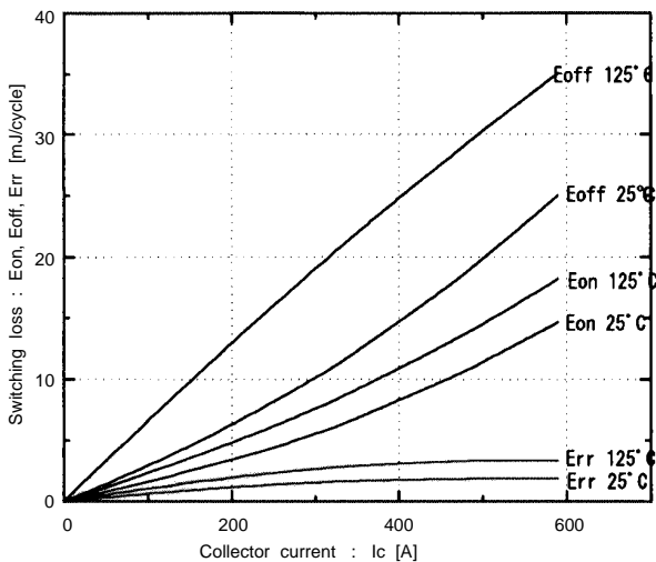
Switching loss vs. Collector current Vcc=300V, RG=4.7 ohm, VGE=±15V
