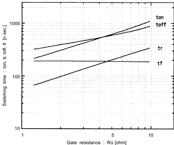
Switching time vs. RG Vcc=300V, Ic=400A, VGE=±15V, Tj=25°C
