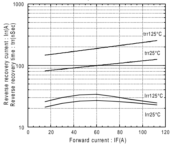
Reverse recovery characteristics trr, lrr vs. IF
