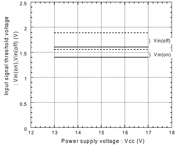
Input signal threshold voltage vs. Power supply voltage T j =25°C (solid line), T j =125°C (dashed line)
