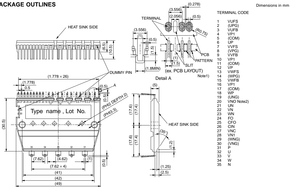
Fig. 1 PACKAGE OUTLINES
