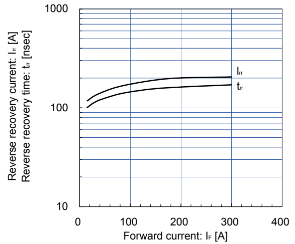
Reverse Recovery Characteristics (typ.) V_{CC}=600V, V_{GE}=\pm 15V, R_G=1.1\Omega, T_J=125^\circ C
