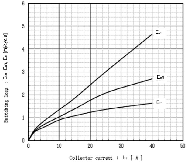
Switching Loss vs. Collector Current (typ.) V_{ce}=600V, V_{cc}=15V, T_j=125^{\circ}C
