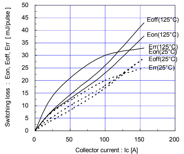
Switching loss vs. Collector current (typ.) V_{cc}=900V, V_{GE}=\pm 15V, R_g=4.7\Omega
